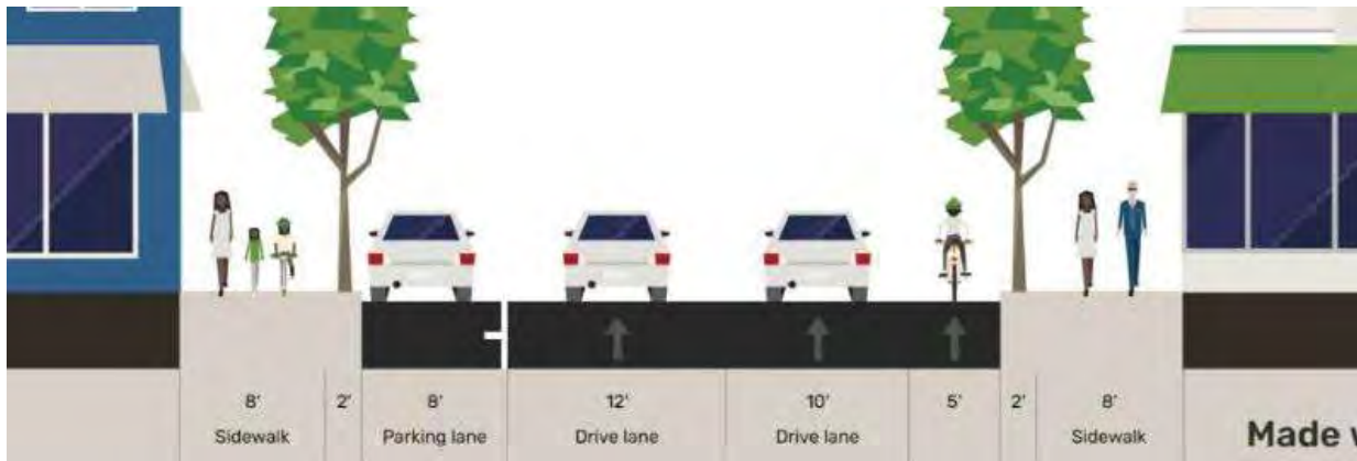
FIGURE 10: MAIN STREET TYPICAL SECTION (ALT 2)
