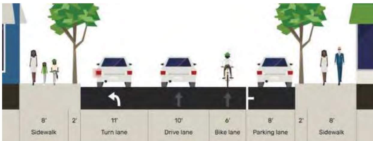
FIGURE8B: ALTERNATE TYPICAL SECTION W/AUX TURN LANE (ALT 1B)
