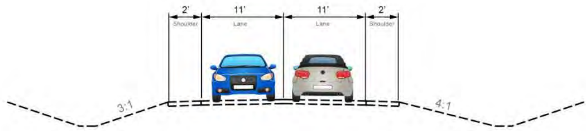
FIGURE 9: 5 TH STREET ROAD COUNTERMEASURE
