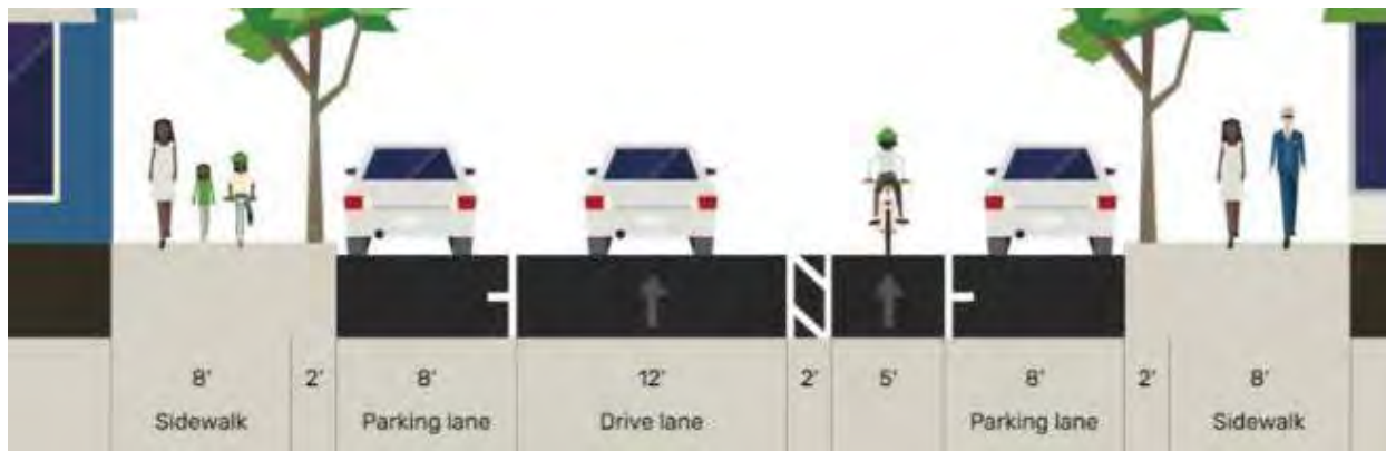
FIGURE 8A: MAIN STREET TYPICAL SECTION (ALT 1A)
